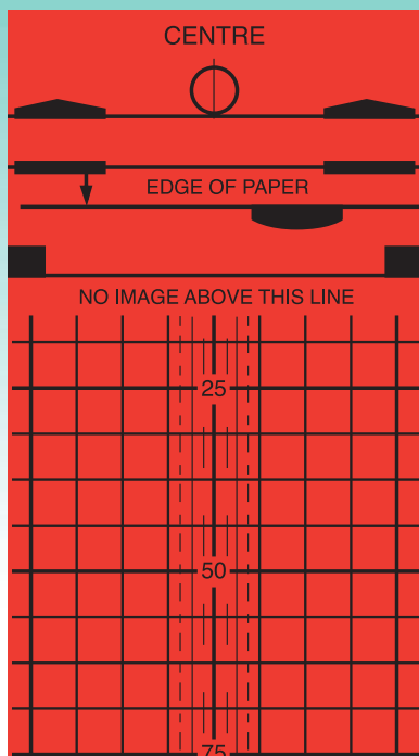
Illustration: GTO 52 Gripper Edge (section only actual size)
